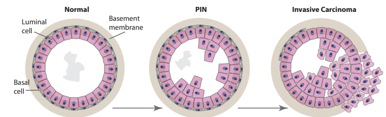
Figure 2. 3D cultures of cells to form cysts (also called spheroids or organoids) also allows us to model the loss of normal tissue architecture that occurs in cancer. For example, the progressive disrupted organisation of Normal, to Prostatic Intraepithelial Neoplasia (PIN), to Invasive Carcinoma typifies prostate cancer progression.
