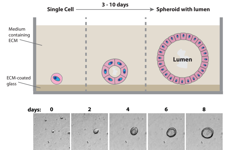
Figure 1. By culturing cells on glass-bottomed chambers coated with extracellular matrix (ECM), we direct the self-assembly of single cells into multicellular spheroid structures with a single, central lumen. This process occurs over 10 days, allowing us to study the dynamics of tissue formation.
